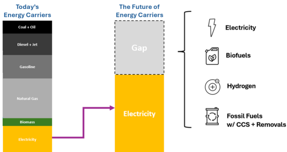
Figure 5 Comparative view of today's dominant energy carriers and a possible future energy mix
