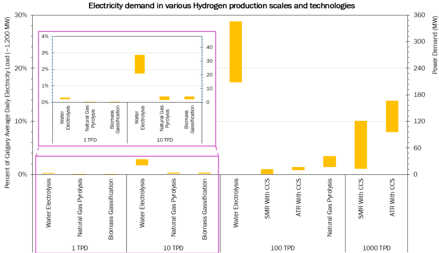
Figure 7 Electricity demand from hydrogen production as a share of Calgary’s 2024 average daily load (~1,200 MW), by technology and production scale
