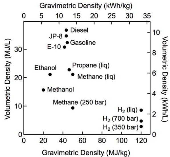
Figure 2 Gravimetric and volumetric energy density of hydrogen compared to other fuels
