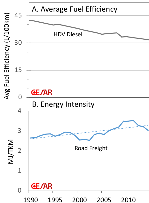
Figure 4.3. Average fuel efficiency (A, L/100 km) of heavy duty road vehicles and trends in energy intensity (B, MJ/TKM) for road freight, marine and rail movement. Fuel efficiency and energy consumption are from Natural Resources Canada [9] and TKM from Statistics Canada [8] with back-casting using CanESS model [14].
