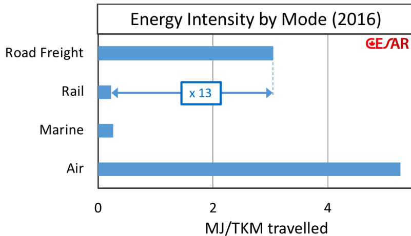
Figure 2.2. Energy intensity for freight transport (MJHHV per tonne-km [TKM] travelled) by mode. Underlying data is from the National Inventory Report [5], Natural Resources Canada [9]-[10], and Statistics Canada [7],[8].
