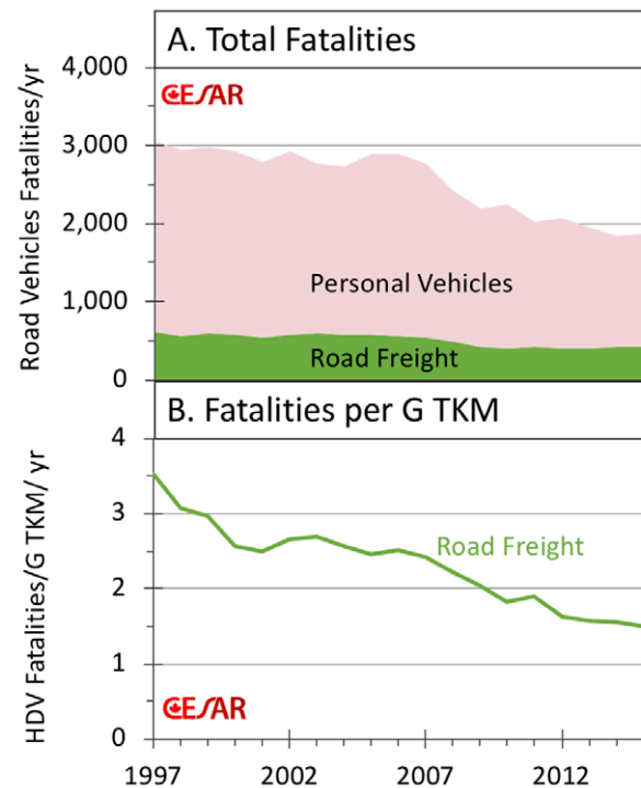
Figure 5.1 Trends in fatalities resulting from motor vehicles in 2015 (A) and Road Freight-Related Fatalities per GTKM Moved (B). Based on data from Transport Canada [37].
