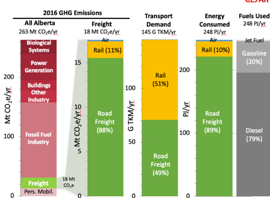
Figure 2.1. An overview of Canada’s (A) and Alberta’s (B) Freight Transportation Sector in 2016, including (left to right) their contribution to total GHG emissions (Mt CO 2 e/yr), modes contributing to GHG emissions, freight moved (t-km travelled), energy used (PJHHV/yr) and fuels consumed (PJHHV/yr). Road freight represents vehicles with a Gross Vehicle Weight Rating (GVWR) of 3.9 tonnes or greater. Data compiled from the National Inventory Report [5] for GHG emissions/energy consumed/fuels used, Statistics Canada [7], [8], and Natural Resources Canada [9]-[10] for transportation demand.
