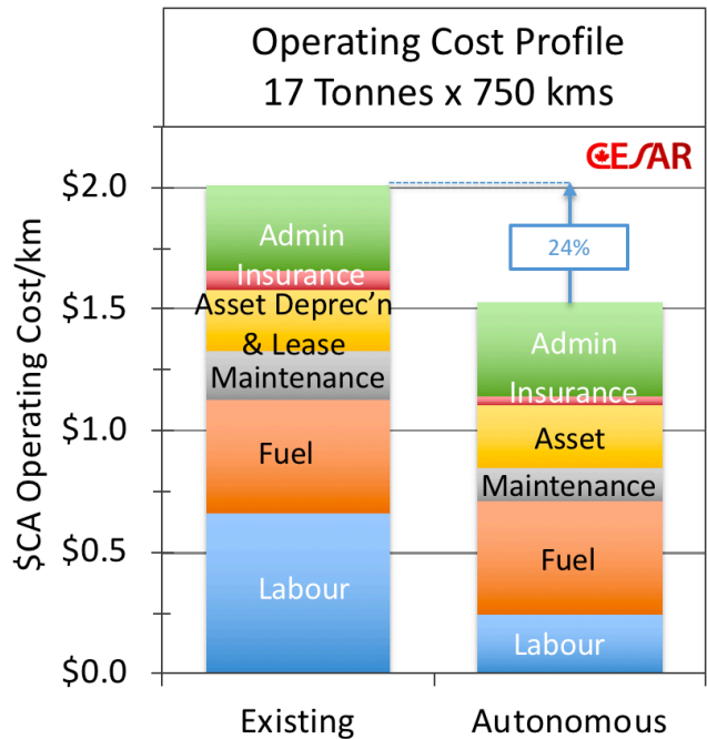
Figure 6.3. Estimated operating cost profile for autonomous electric HDV. Calculated from Figure 4.4C data assuming (a) drivers represent 70% of salary, wage and benefit costs and this portion of the cost is reduced by 90%; (b) asset cost increases are fully offset by increased use rate; (c) 30% lower maintenance cost; (d) no change to fuel and G&A costs.
