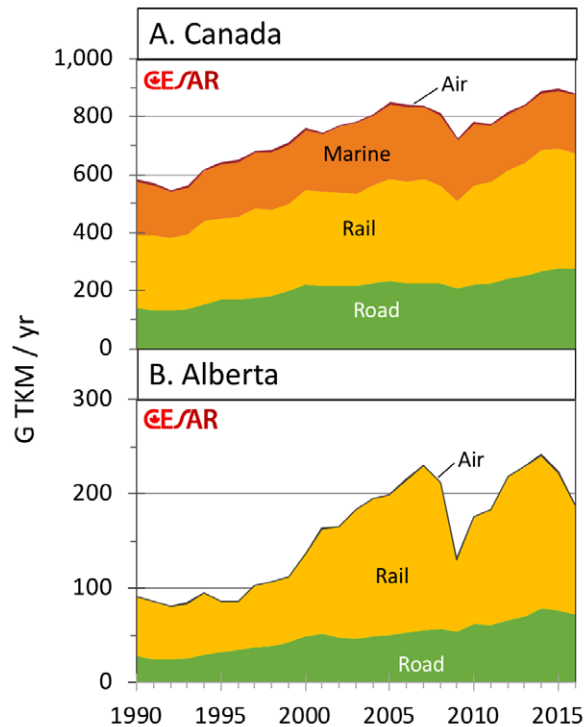
Figure 3.1. Freight Transportation Activity in billion tonne-km (GTKM) travelled per year by mode for Canada (A) and Alberta (B). Canada data from Statistics Canada [8] and Natural Resources Canada [9] with truck demand backcast for years prior to 2004 using the CESAR based on GHG data from the National Inventory Report [5].
