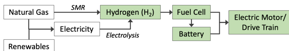
Figure 6.2. Zero-emissions electric truck options. The shaded boxes represent technologies that are aboard the vehicles; steam methane reforming [SMR].
