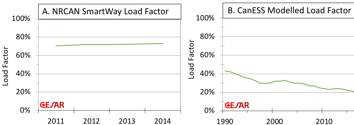
Figure 4.6. Load Factor, SmartWay Reported (A) and Modelled (B). Load Factor as a Product of Capacity Utilization and Loaded Kilometres Travelled. NRCAN SmartWay collects capacity utilization and empty kilometres from its members [26], and CanESS load factor is determined based on a combination of Statistics Canada data sources for transportation, energy use and stock data [14].
