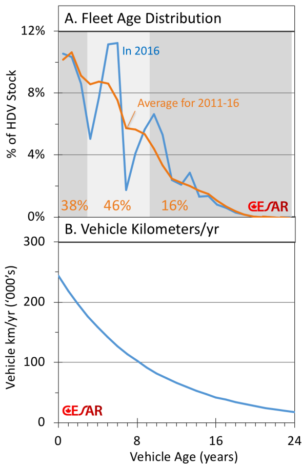
Figure 4.2. Fleet age distribution (A) for HDV kilometers travelled (VKT) per year by vehicle age (B). Estimates obtained from the CanESS model [14] [23].
